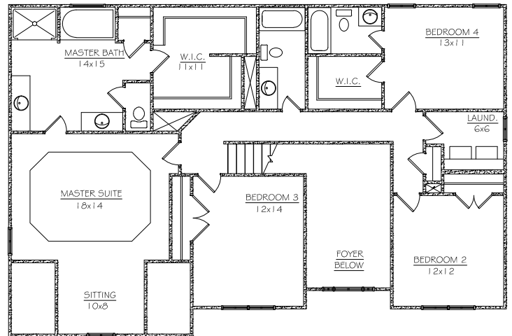
2ND FLOOR
