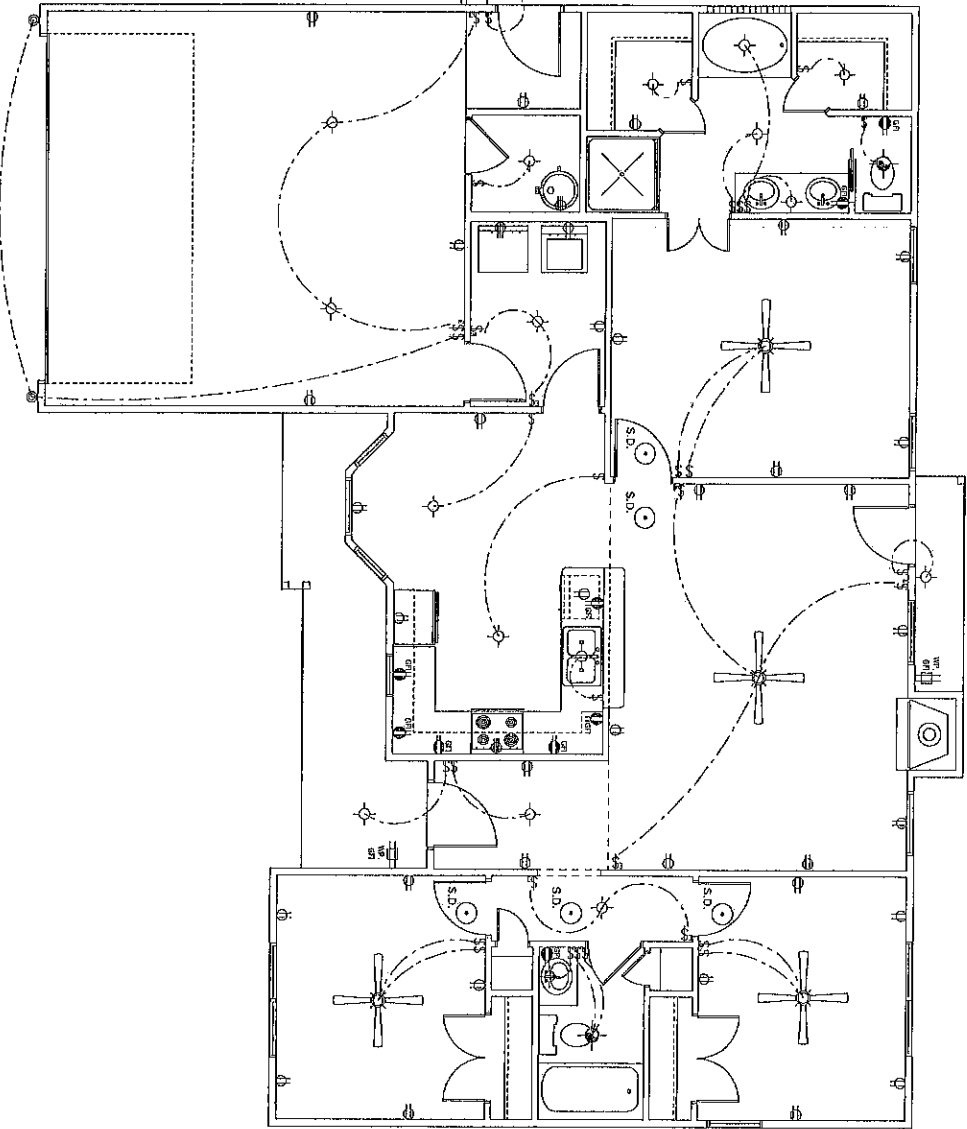
ELECTRICAL PLAN SCALE: 1/4" = 1'-0"
