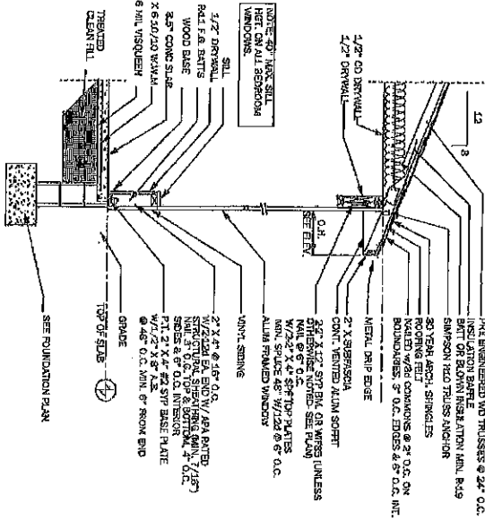
TYPICAL WALL SECTION EXTERIOR FRAME SCALE: 1/2" = 1'-0" 9 S6
