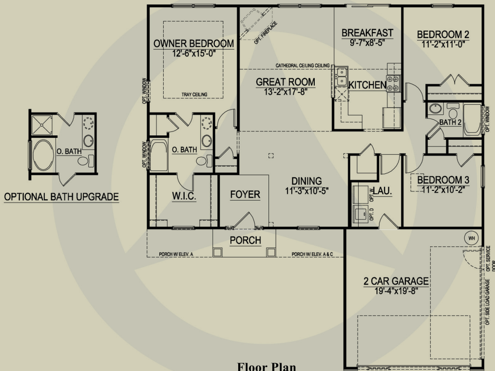
Floor Plan
