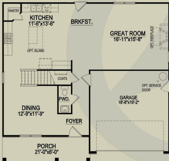
Floor Plan
