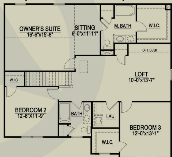
Second Plan
