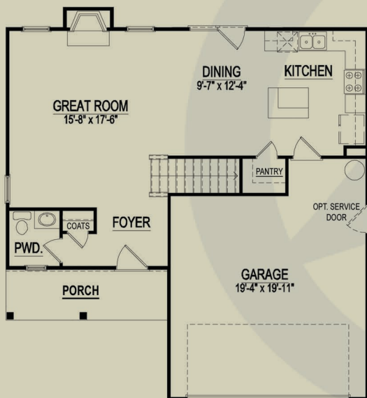
Floor Plan
