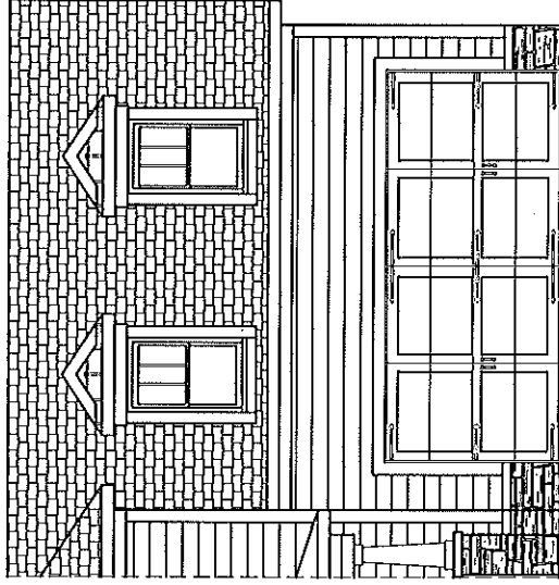
OPTIONAL TWO-CAR GARAGE ELEVATION B
